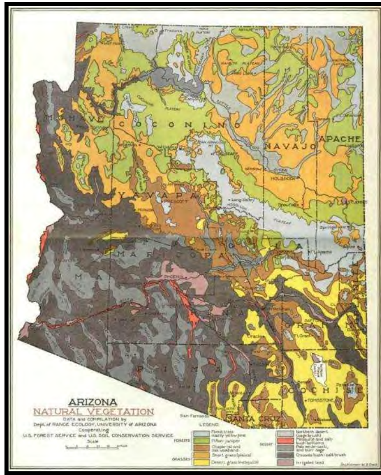
Figure 35. Nichol's 1937 map of Arizona's natural vegetation.
