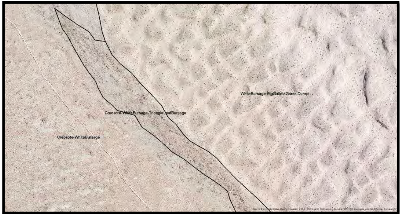
Figure 123. Above, an image of the west side of the Mohawk Dunes, of an area about 2.4 km (1.5 miles) across. Note characteristic crest/swale of dune landform.
