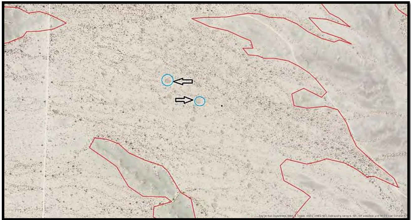
Figure 107. Blue circles show large hummocks of club cholla near Foothills Blvd (on left).
