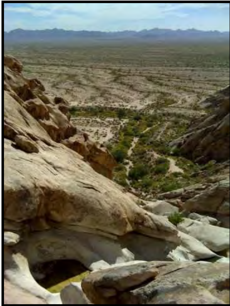
Figure 20. The view east from the highest of the Tinajas Altas , or high tanks. The track of the Camino del Diablo can be seen approaching from the back right. Water is in the top tank, half-shaded by the granite wall.
