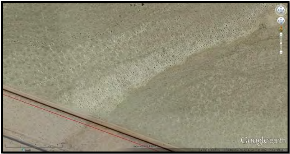
Figure 64. Image showing sand ridge in center of photo, the pale slash running southwest to northeast. This is along the international border, south of the Butler Mountains.
